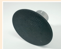
Round sieve nozzle, Ø 260 mm Article No: 107.276
